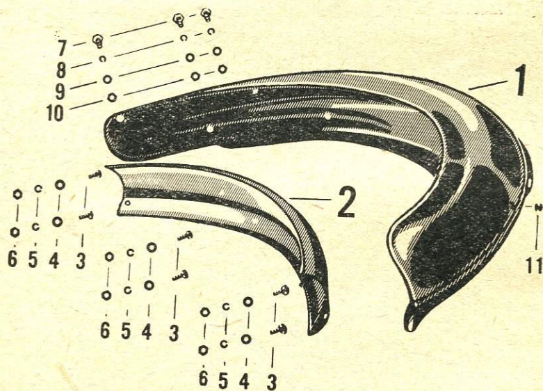
Rear Wheel Mudguard - Hinterer Kotflügel - Garde-boue AR - Guardabarros trasero
