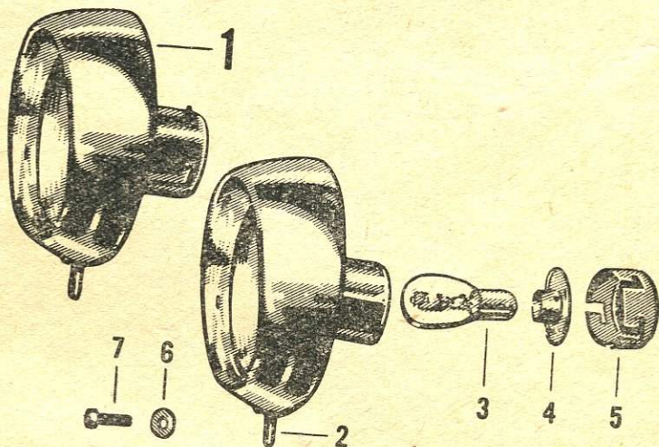
Headlamp - Scheinwerfer - Phare - Faro
