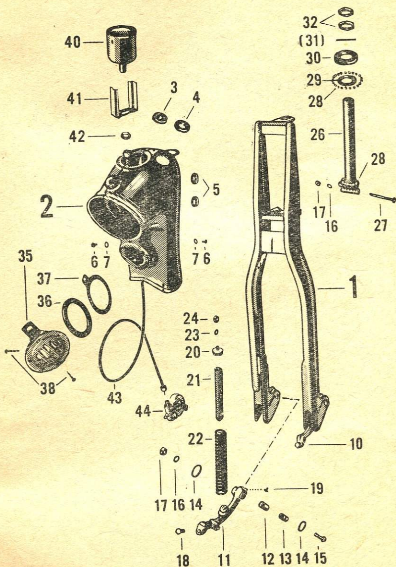
Front Wheel Fork - Fordergabel - Fourche avant - Horquilla delantera
