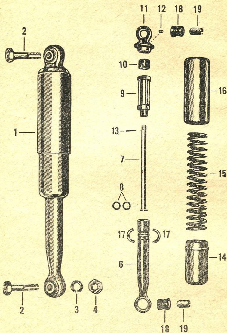
Telescopic Shock Absorber - Elast. Teleskop - T  lescope souple - Telescopio elastico
