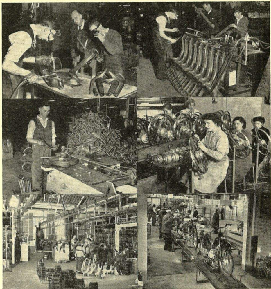
BUILDING THE NORMAN NIPPY: These pictures, taken at the Ashford works of Norman Cycles, Ltd., are of some of the processes which go into the production of the Nippy moped. They are (top, left), welding the tank and main-frame pressings; (top, right), welding and final frame-welding section; (centre, left), exhaust pipe and handlebar bending section; (centre, right), moped wheel building section; (bottom, left), enamelling by the Ransburg electrostatic process; and (bottom, right), final assembly conveyor.
