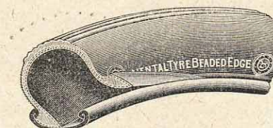
Continental (beaded edge) Tyre.
