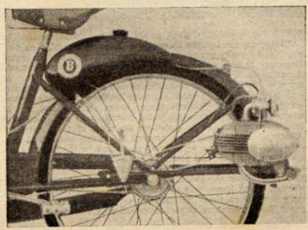
Yet another position for the engine! For his new 48 c.c. "B" cyclemotor, Ing. Giuseppe Benelli has chosen this outside-the-wheelbase position.
