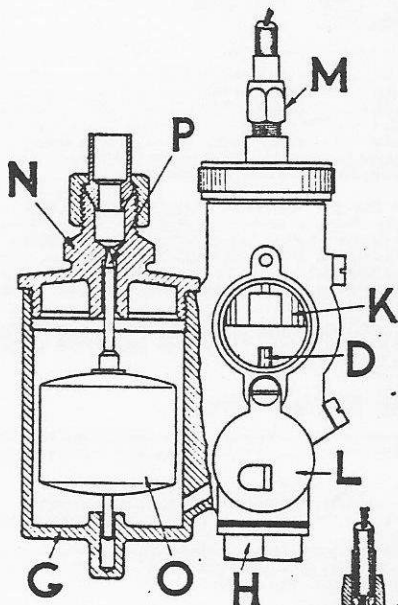
Section through Float Chamber.
