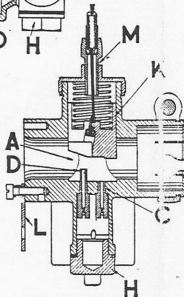
Section through Jet Chamber showing position of jets.
