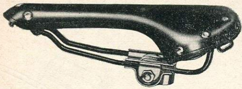
BROOKS CHAMPION SPORTS SADDLE No. B17. Swallow. Two-wire. Size 11" x 6" x 3 1/8". Weight 1 lb. 9 ozs. S5/4500 Chrome finish ... each 67/6
