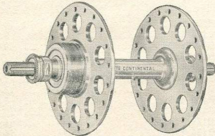
"AIRLITE-CONTINENTAL" REAR HUB
