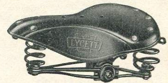
LYCETT'S TOURIST SADDLE No. L71. Three-coil. Size: 10'' \times 8\frac{1}{4}'' \times 3\frac{7}{8}'' . Weight, 2 lb. 2 oz. Gent's Model. S77/1400 Enamel ... .. each 21/- No. L71L. Ladies' Model. Size: 9\frac{3}{4}'' \times 8\frac{1}{4}'' \times 3\frac{7}{8}'' . S78/1400 Enamel ... .. each 21/-
