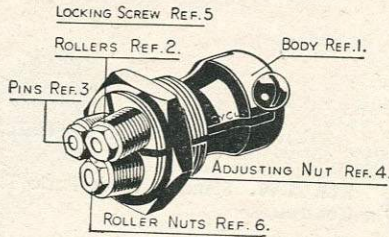
CYCLO SPOKE THREAD ROLLING HEADS
