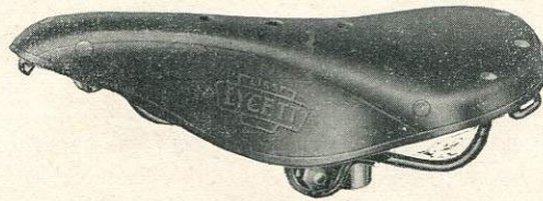
LYCETT'S STANDARD SADDLE No. L15. Two-wire. Sports Model with solid leather top. Black enamel. Size: 11'' \times 6\frac{3}{4}'' \times 3\frac{1}{8}'' . S61/1600 Enamel ... .. each 24/- S62/1708 Chromium ... .. each 26/6
