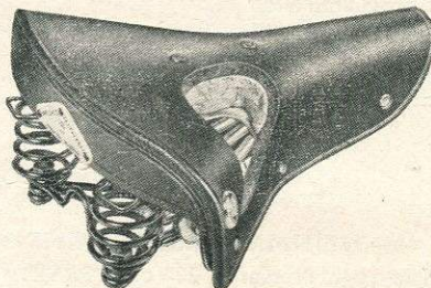
WRIGHTS FEATHERBED SADDLE No. 505. A sprung mattress saddle with felt underlay, airfoam interior and soft leather anti-friction lining. Vynide waterproof seat corner-guard protected. Ladies' and Gent's Models. Enamelled. S25/1804 ... each 27/6
