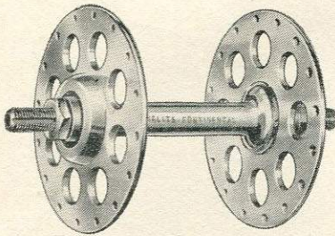
"AIRLITE-CONTINENTAL" FRONT D.S. HUB
