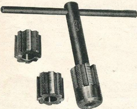
CYCLO BOTTOM BRACKET CLEARING TAP No. 123. R. and L. hand thread, 1\frac{3}{8} " x 24T. W104/Trade ... .. each 12/1
