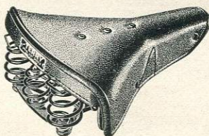
TERRY'S EXTRA COIL SADDLES With patent suspension. Automatically adjusts to carry any weight rider. No. 1087X. Ladies' Model. Size: 9\frac{1}{2}'' \times 8\frac{1}{2}'' . S57/1608 ... .. each 25/- No. 1086X. Gent's Model. Size: 9\frac{1}{2}'' \times 10\frac{1}{2}'' . S58/1608 ... .. each 25/- Replacement Top S59/808 ... .. each 13/-
