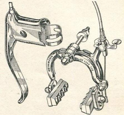
WEINMANN LIGHTWEIGHT CABLE BRAKES
