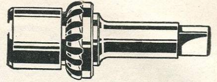
CYCLO HEAD LUG REAMER No. 119. Standard type complete with holder and revolving guide. W118/Trade ... .. each 24/2
