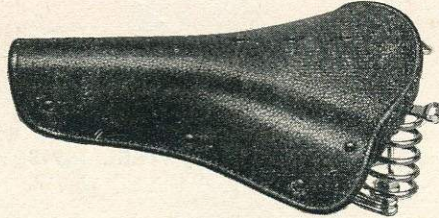
BROOKS MATTRESS SADDLE No. B22. Multi-mattress spring construction. Four-wire bracket, with two rear coils. Size: 10 3/4" x 9 1/4" x 3 1/8". Chrome plated. S14/1804 ... each 27/6
