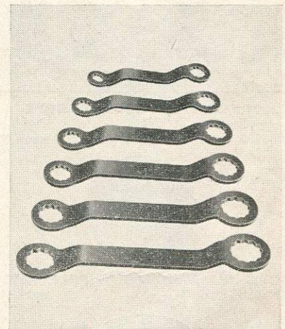
LINCO No. 8 RING SPANNER SET Set of six Whitworth ring spanners. Sizes: \frac{1}{8} " \times \frac{3}{16} ", \frac{3}{16} " \times \frac{1}{4} ", \frac{1}{4} " \times \frac{5}{16} ", \frac{5}{16} " \times \frac{3}{8} ", \frac{3}{8} " \times \frac{7}{16} ", \frac{7}{16} " \times \frac{1}{2} ". S252/500 ... .. per set 7/6
