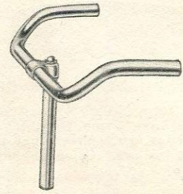
PHILLIPS HANDLEBARS No. 85. Raised. 18" wide. 20" wide to order. Chromium plated. H92/901 ... each 13/8
