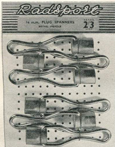
"RADSPORT" 14mm. PLUG SPANNERS Clean, bright finish, with swivel handle. 6 per card. R7/900 card ... .. each 2/3
