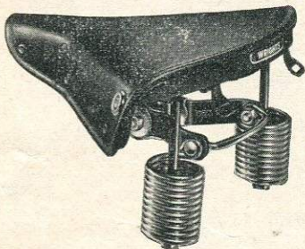
WRIGHTS POWER-CYCLE SADDLE No. S65/3. For Motorised Bicycles. Sprung mattress interior with thick felt underlay. Vynide waterproof seat, size, 10 3/4" x 11 1/2". Shock absorbing tension coils, double girder pivoted frame and chromium-plated rear coils and clip. Enamelled. S26/1804 ... each 27/6
