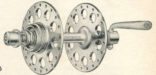
B.H. "AIRLITE-CONTINENTAL" FRONT HUB
