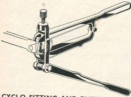
CYCLO FITTING AND EXTRACTING TOOL No. 147. For Crank Cotter Pins. W100/Trade ... .. each 33/-
