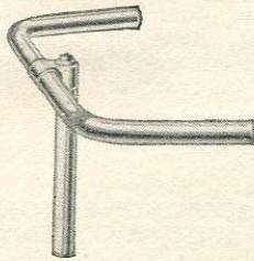
PHILLIPS HANDLEBARS No. 86. Standard flat, 18" wide. 20" wide to order. Chromium plated. H89/901 ... each 13/8
