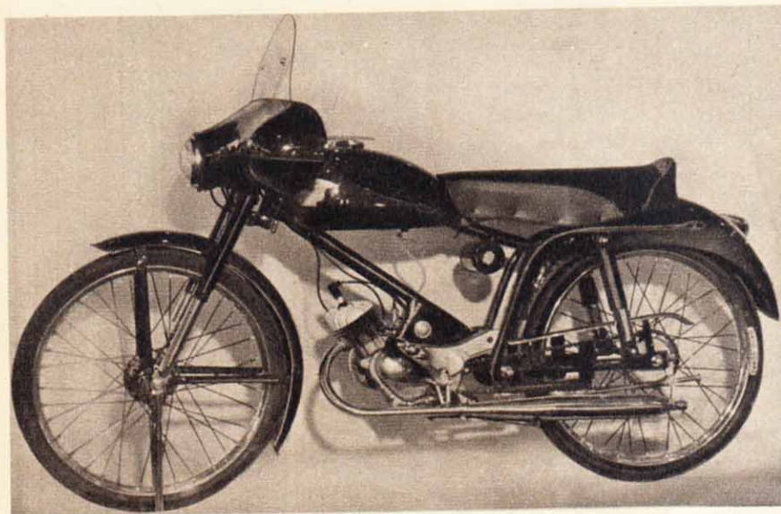
Rear-sprung and with a 48 c.c. engine, this is a typical example of "ciclomotore" such as is selling readily in Italy. It is the Vittoria-N.S.U. "Solitude" model.
