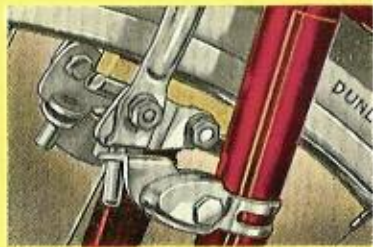
RALEIGH BELL CRANK. Careful design, combined with extreme neatness, provide a smooth and very efficient rear centre pull roller lever brake.
