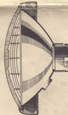
S0065 Lamp Front Unit (in section)
