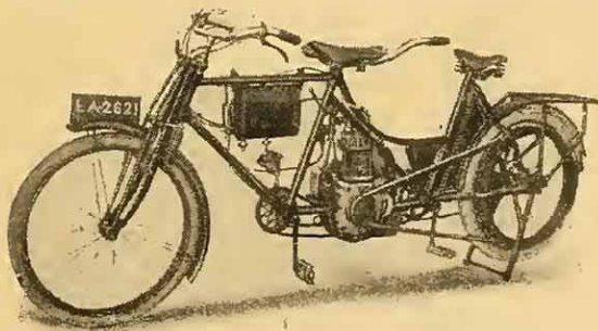
An old tandem motor cycle, modernised by J. J. W. Pater, of Bedford, and still doing good service. The engine is an old pattern 2\frac{1}{2} h.p. Minerva, to which a magneto and B. and B. carburetter have been fitted.
