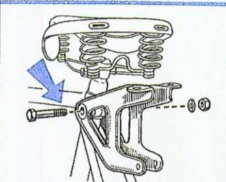
4 A specially strong saddle bolt is supplied that replaces the normal saddle bolt.
