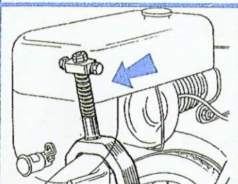
5 Coil spring suppresses shocks over bad road surfaces.
