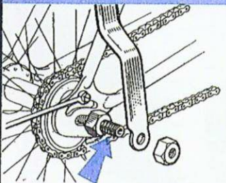
1 Special extension nut is provided for fitting rear wheel. Speed gear is unaffected.
